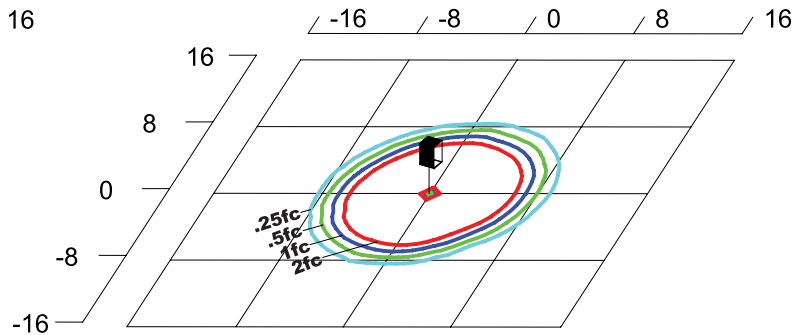
BOGRLQF1X15U5K Type V Grid in feet, Mounting Height = 3.5 ft.
