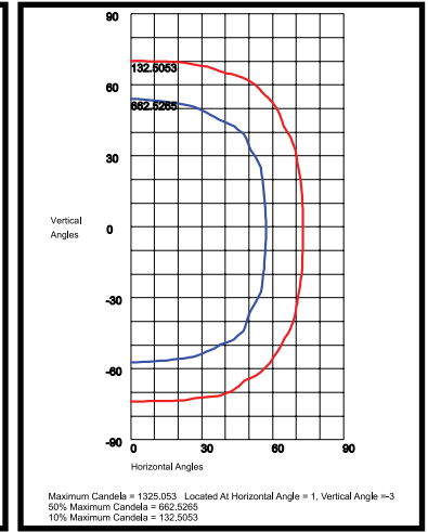
KH25QF1X36UHAC 115°H x 110°V Beam, NEMA 7H x 7V
